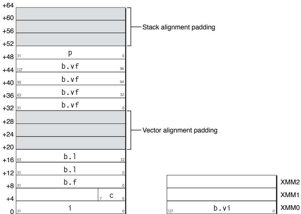
Figure 3 Argument assignment with structure and vector arguments
