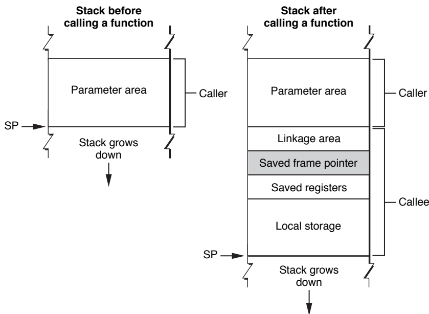
Figure 1 Stack layout
